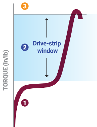
1 Thread-forming begins
